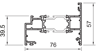
SPW769717G SPW769717W SPW769717DWG flush deep outerframe
