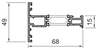
SPW712713G SPW712713W SPW712713DWG flat faced vent
