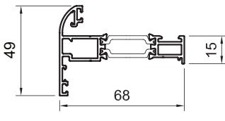
SPW710713G SPW710713W SPW710713DWG radius vent
