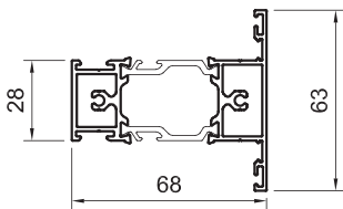
SPW767768G SPW767768W SPW767768DWG deep screwport transom/mullion
