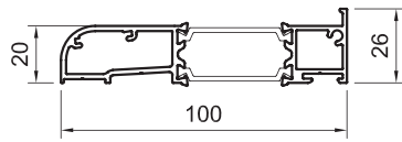
SPW790753G SPW790753W SPW790753DWG 100mm cill
