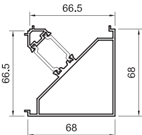
SPW740748G SPW740748W SPW740748DWG 90° corner post
