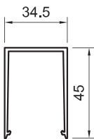
PUR034G PUR034W PURe add on reinforcing cap
