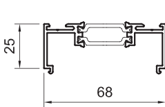
SPW730730G SPW730730W SPW730730DWG 25mm add on
