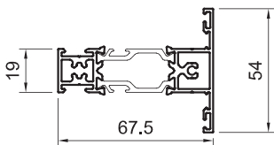
SPW706707G SPW706707W SPW706707DWG transom/mullion (screwport)
