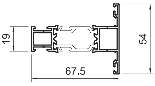
SPW703704G SPW703704W SPW703704DWG transom/mullion (shearblock)
