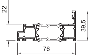
SPW764701G SPW764701W SPW764701DWG flush outerframe
