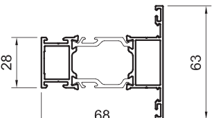
SPW765766G SPW765766W SPW765766DWG deep shearblock transom/mullion
