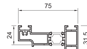
SPW255256G SPW255256W SPW255256DWG floating mullion lock adapter
