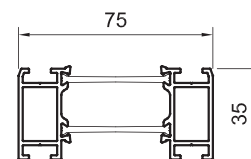
SPW253253G SPW253253W SPW253253DWG floating mullion
