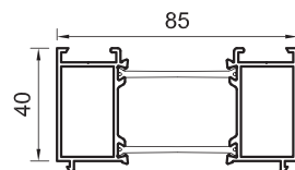
SPW6024024XG SPW6024024XW SPW6024024XDWG 40mm add on (85mm frame)
