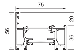
SPW252233G SPW252233W SPW252233DWG flat faced door stile
