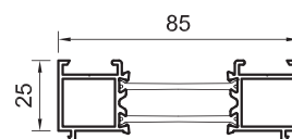
SPW65353XG SPW65353XW SPW65353XDWG 25mm add on (85mm frame)
