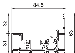
SPW231230G SPW231230=W SPW231230DWG outerframe
