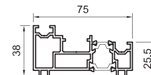
SPW236237G SPW236237W SPW236237DWG master O/O lock stile
